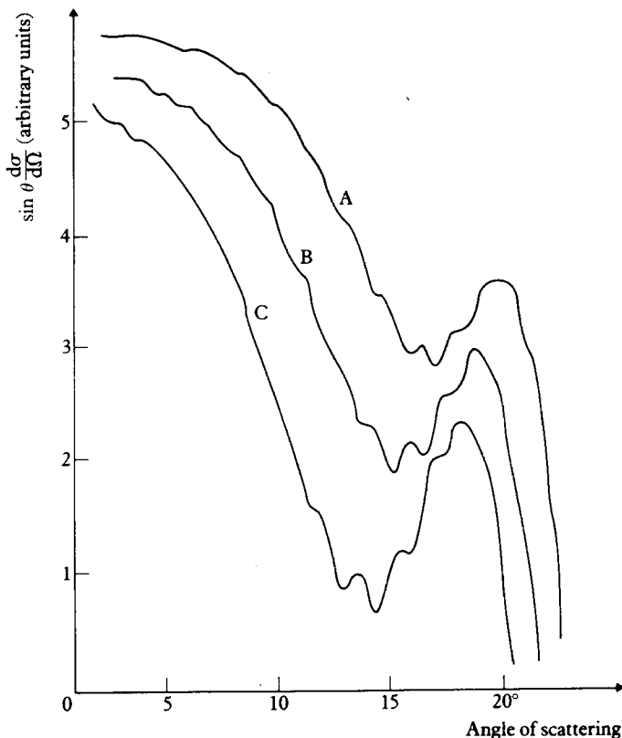
13.7 The differential cross-section for the elastic scattering of sodium atoms by krypton atoms measured by Barwig, Buck, Hundhausen and Pauly for relative velocities of (A), 767 m/s (B) 817 m/s (C) 870 m/s. Quantum mechanical interference effects are seen in the region of the rainbow angle. At smaller angles ( \theta < 2^\circ ), the cross-section follows the \theta^{-7/3} law, for scattering by the potential V(r) \cong -A/r^6 (see equation [13.38]).
